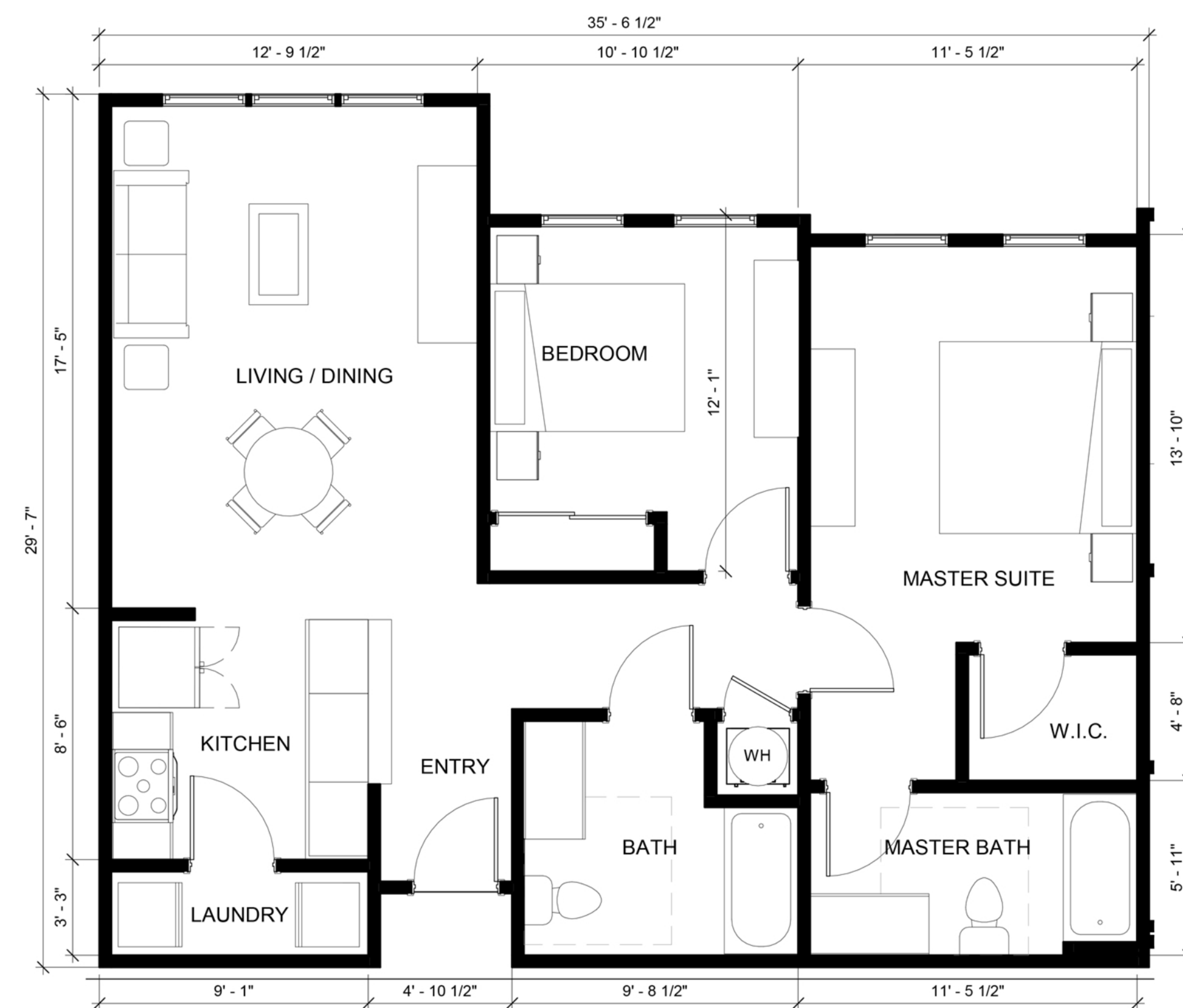
2 2 BEDROOM UNIT (925 SQ FT) 1/4" = 1'-0"
