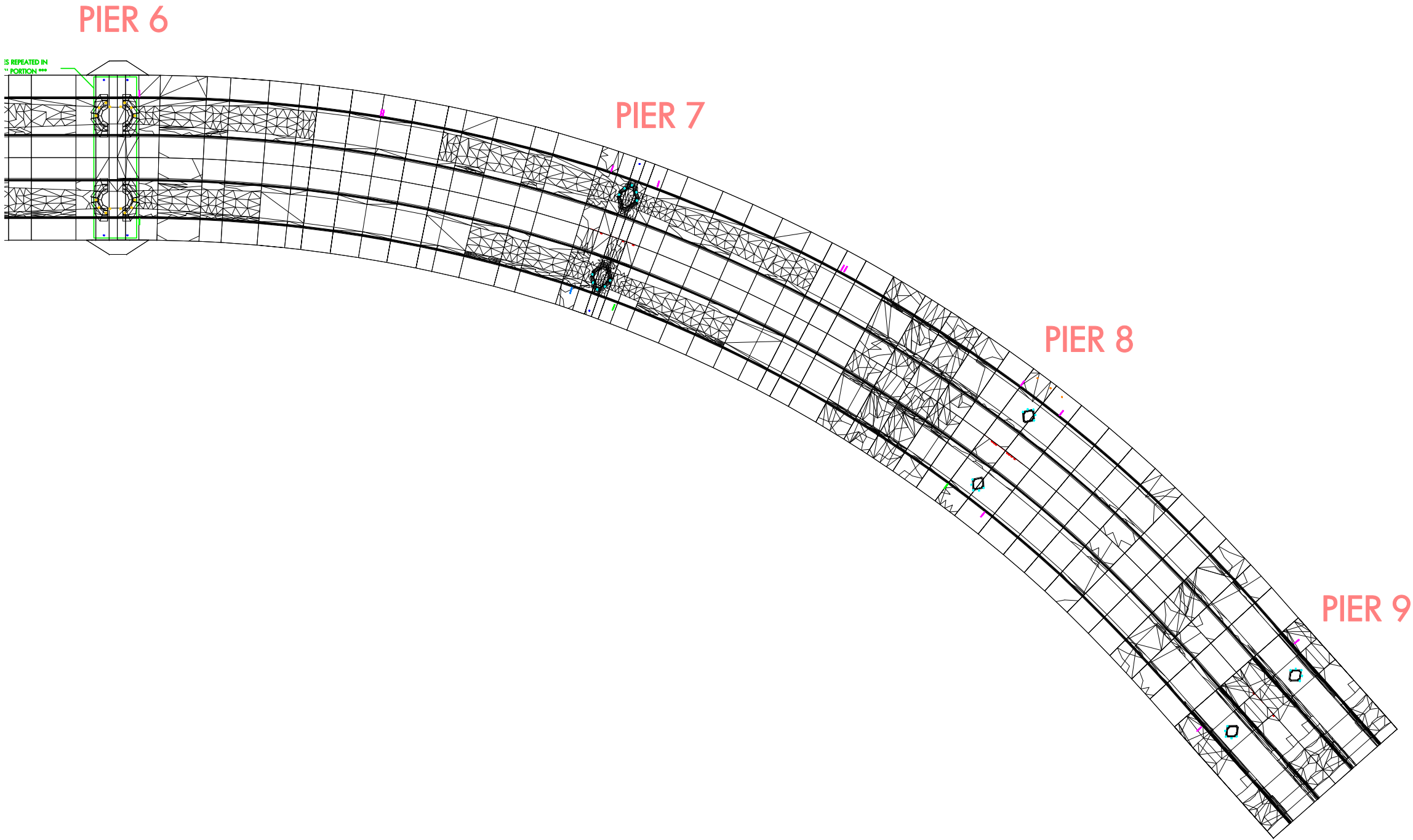
PLAN VIEW
