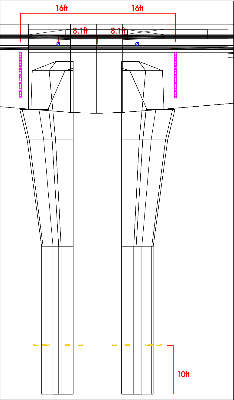
ELEVATION VIEW (PIER 5 & 6)
