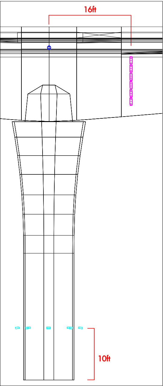
ELEVATION VIEW (PIER 4)
