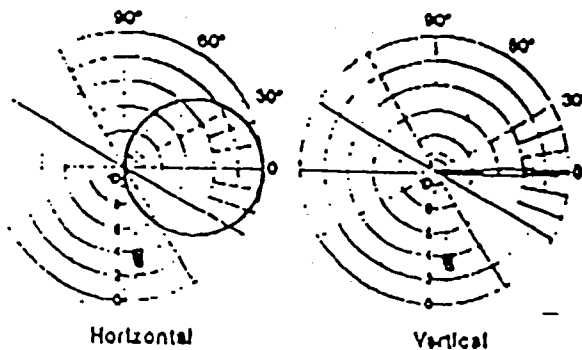
Radiation Patterns (Relative Field Strength) Bandwidth
