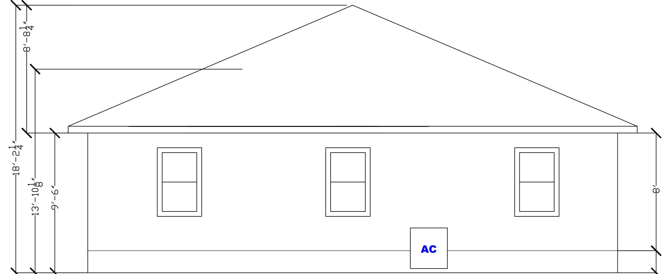
D Side Elevation
