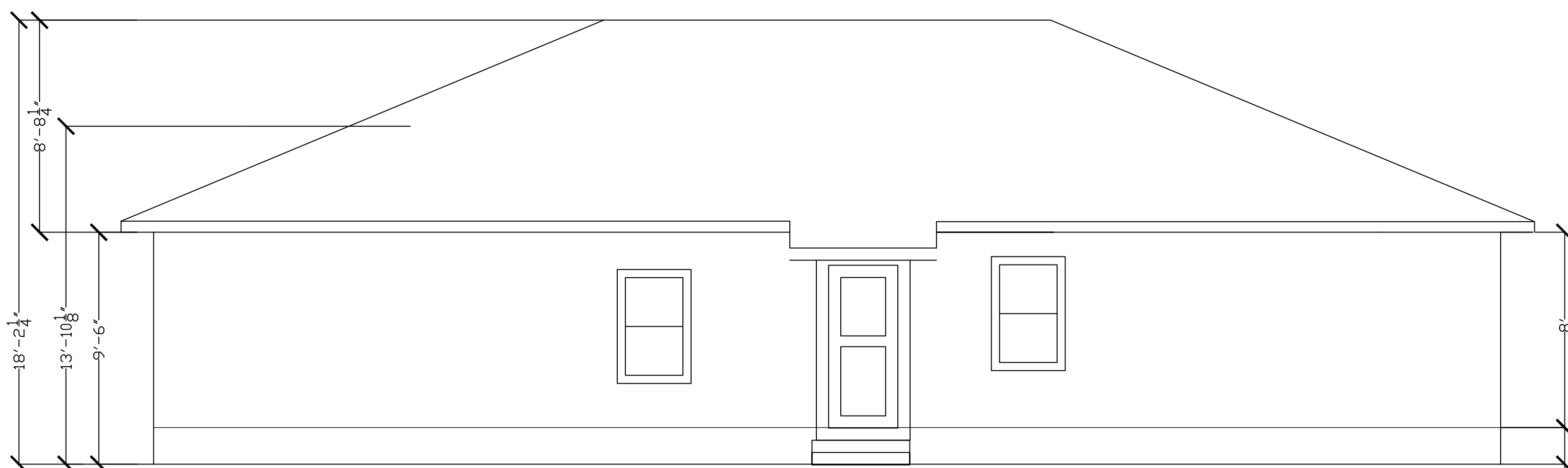
A Rear Elevation
