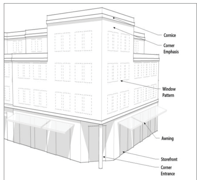
Figure 32. Corner Treatments
