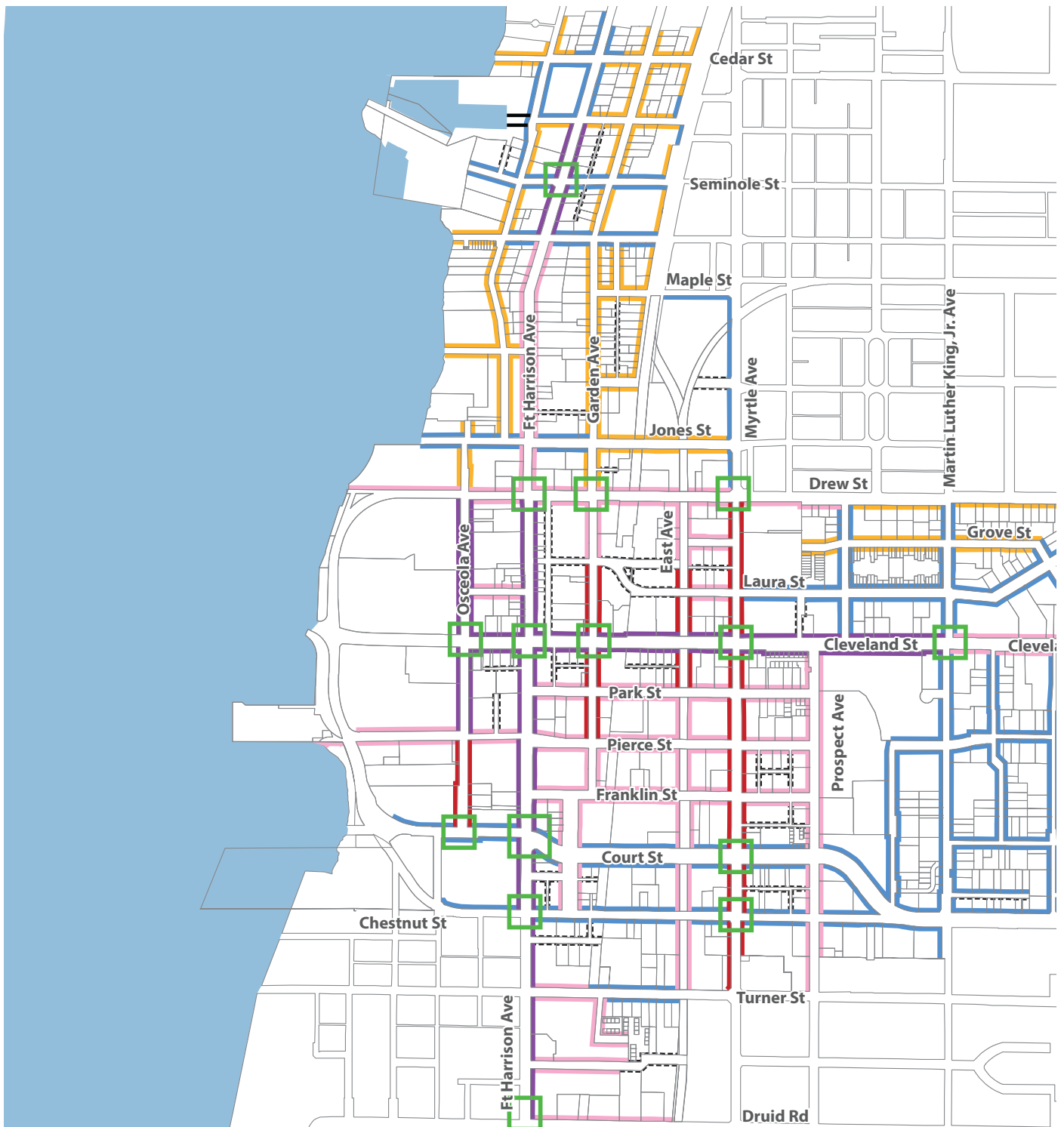
Figure 2. Regulating Plan – Street Types and Key Corners
